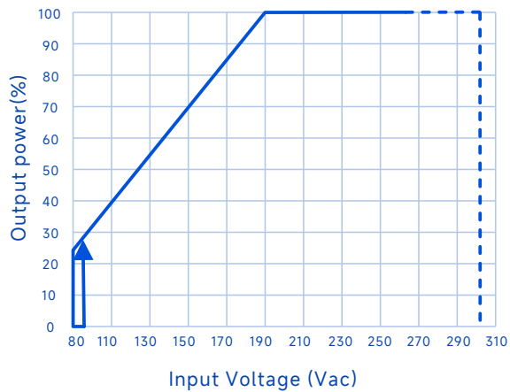
O/P Power Vs. Input Voltage (Ta Max.55°C)
